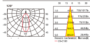
Luminaire photometric diagram:
