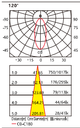
Luminaire photometric diagram:
